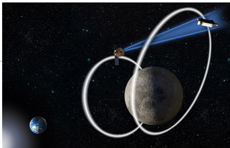
The image depicts one possible cislunar orbit, where the Air Force Research Laboratory's Oracle spacecraft will collect observations of resident space objects in the region near the Moon. These observations will be cataloged and used to maintain space situational awareness in support of the space community and help enable a free and open environment for commerce and space exploration for all. (Image credit / AFRL)
